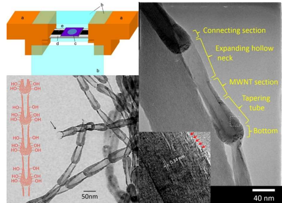
Figure 1 (Left top) Schematic of the synthesis chamber of the submarine-style CVD apparatus. (a) Electrodes, (b) borosilicate glass plates, (c) catalyst-loaded silicon substrate, (d) substrate support, and (e) carbon plate heater. (Left bottom) TEM image of carbon nanopot fibers. A schematic of a carbon nanopot fiber hydroxylated at the graphene edges is also exhibited. (Right) TEM image of carbon nanopots. The inset is a magnified view of the section indicated in the tapering tube part. The arrows point to the graphene edges. After H. Yokoi et al., J. Mater. Res. 31 , 117 (2016). (Cop.: Materials Research Society, Reprinted with permission)
