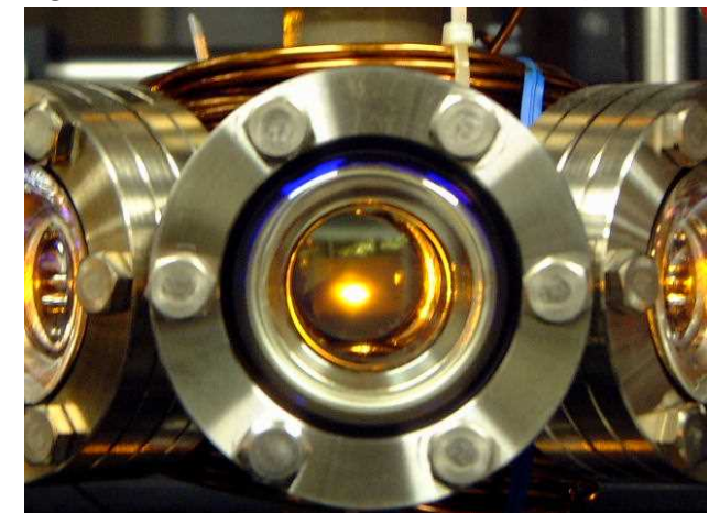
Figure 2 Laser-cooled Na atom cloud
