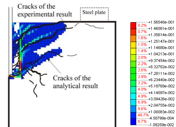
Figure 2. Comparison between experimental crack pattern and analytical one.
