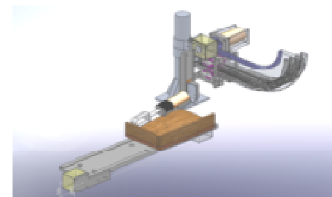
Fig.4 Meal support system
