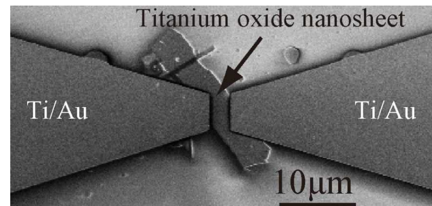
Figure 2 SEM image of titanium oxide nanosheet device
