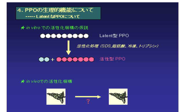
Figure 3 Activation mechanism of latent PPO
