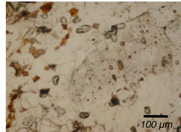
Figure 2. Photo of olivine with abundant fluid inclusions.
