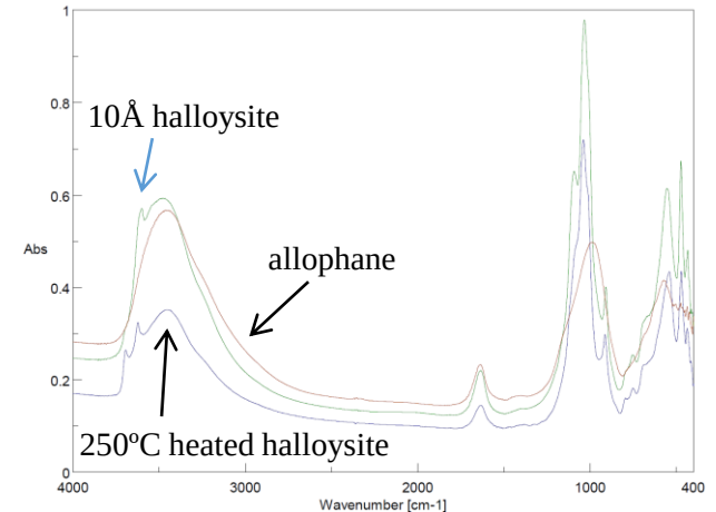
Figure 1 FTIR spectra of altered swellable clay
