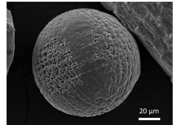
Figure 2 Spherule produced by quick quench experiment
