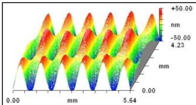
Figure 1 Bio-inspired surface by MWB
