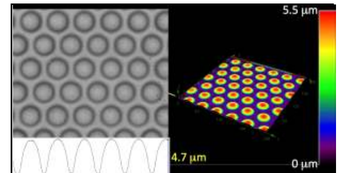
Figure 3 Creation of lotus leaf structure
