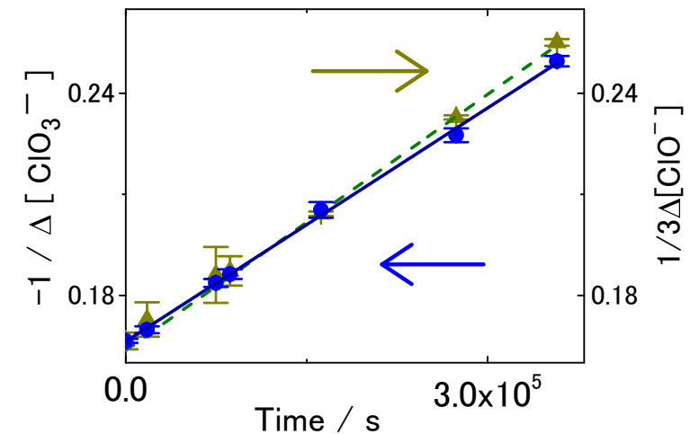
Figure 1. Change of chlorate and hypochlorite.
