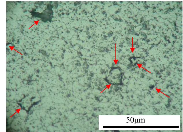
Figure 1 Creep Damage of High-Chromium Steel
