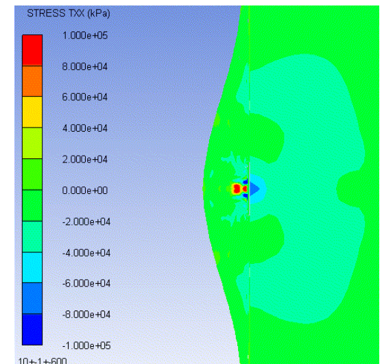
Figure 3 Image of numerical analysis of a droplet impact
