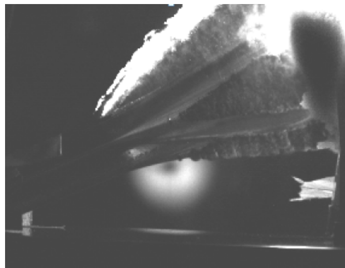
Figure 2 Photograph of metal jet from Linear shaped charge
