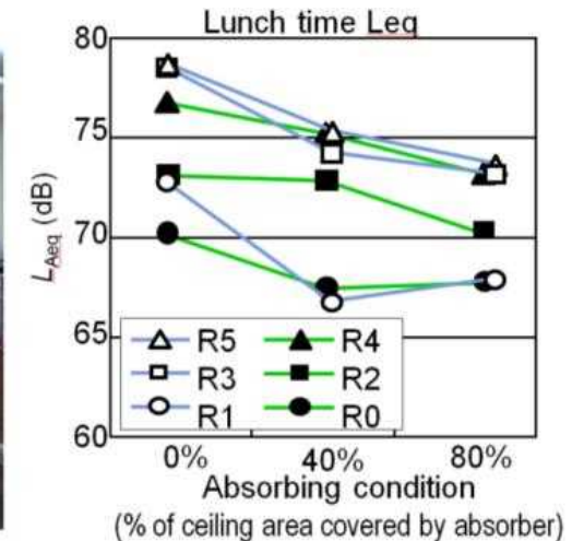
Figure 1 Experiment with installation of sound absorptive material on the ceiling
