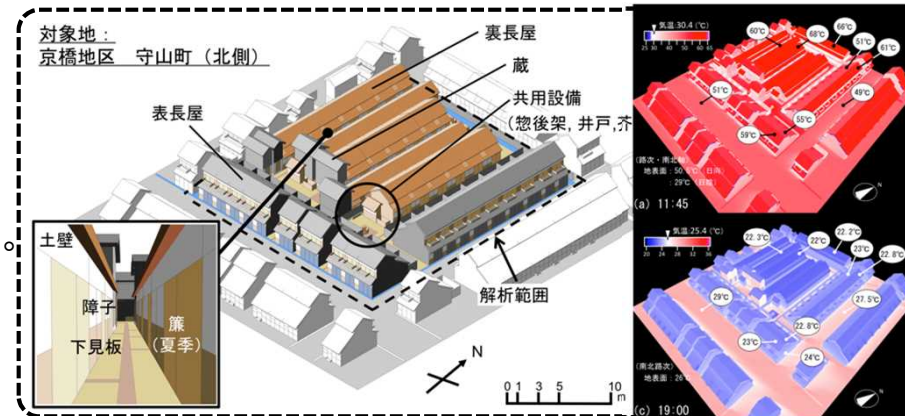
Figure 1 Distribution of surface temp. in Edo (early modern)
