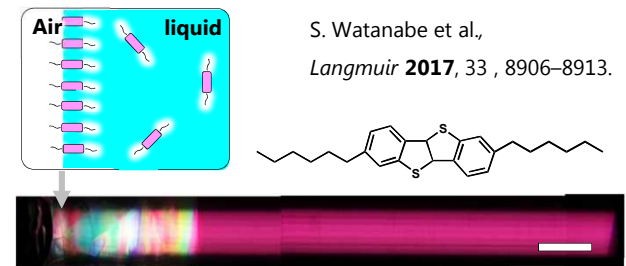
Figure 1 Optical microscope image of a single crystal of an organic semiconductor molecule in glass capillary.
