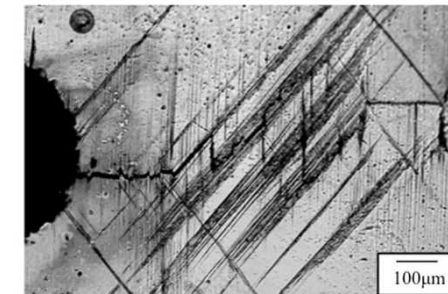
Figure 2 Fatigue crack growth in Mg.
