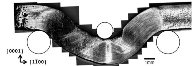
Figure 1 Bending deformation of Mg single crystal.
