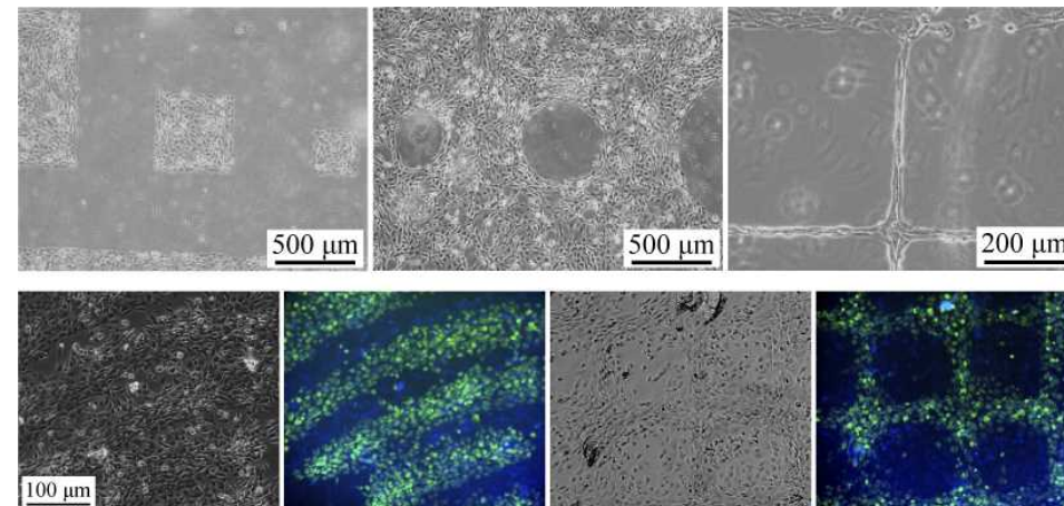
Figure 2 Created cell micropattern and artificial tissues
